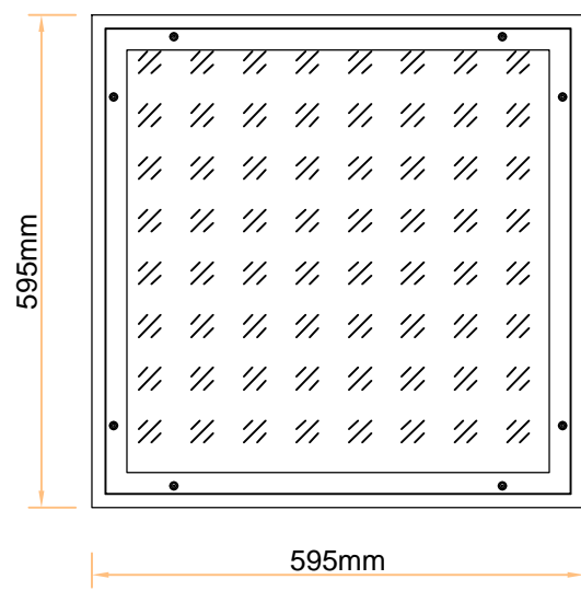
BOTTOM PLAN VIEW Scale 1:10
